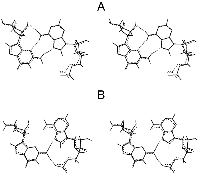
FIGURE 3 Comparison of two low energy subtopologies of the tandem G:A-mismatches in the sheared arrangement. The arrangement in form I (continuous line, hydrogens included) is characterized by three strong (small distance) hydrogen bonds between adenine (strand 1) N 7 and guanine (strand 2) H 2 N 2 , between adenine H 2 N 6 and guanine N 3 , and between adenine H 1 N 6 and the O 2 of guanine (indicated as short dashed lines). This topology is similar to the topology found experimentally in the NMR structure by SantaLucia and Turner (1993) and for example also in the x-ray structure of the hammerhead ribozyme (pdb-entry 1hnh, Pley et al., 1994). The G:A basepair formed by nucleotides G120 and A90, respectively, of the hammerhead ribozyme structure is superimposed (dashed line in A, no hydrogens included) on the calculated type I basepair. In the alternative low energy sheared G:A basepairing arrangement (type II, continuous line in B, hydrogens included) two short distance hydrogen bonds (between N 7 of adenine and H 2 N 2 of guanine and O 1 P of adenine and H 1 N 2 of guanine) are formed (short dashed lines in B). A G:A sheared basepair similar to subform II is also present as a closing basepair of the GAAA tetraloop in the hammerhead x-ray structure (nucleotides G21 and A24 of pdb-entry 1hnh, dashed lines in B, no hydrogens). In A and B, the guanine corresponds to the left base of the basepairs.
